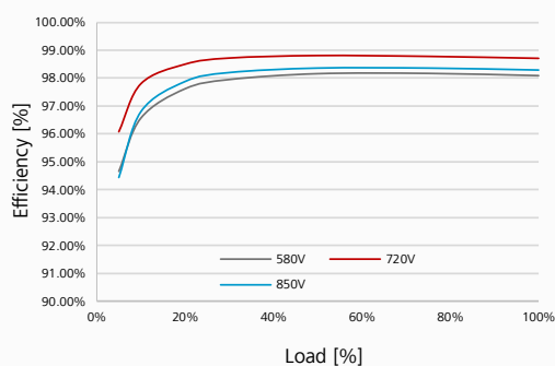
Efficiency Curve
