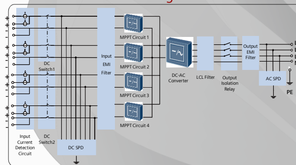
SUN2000-36KTL
